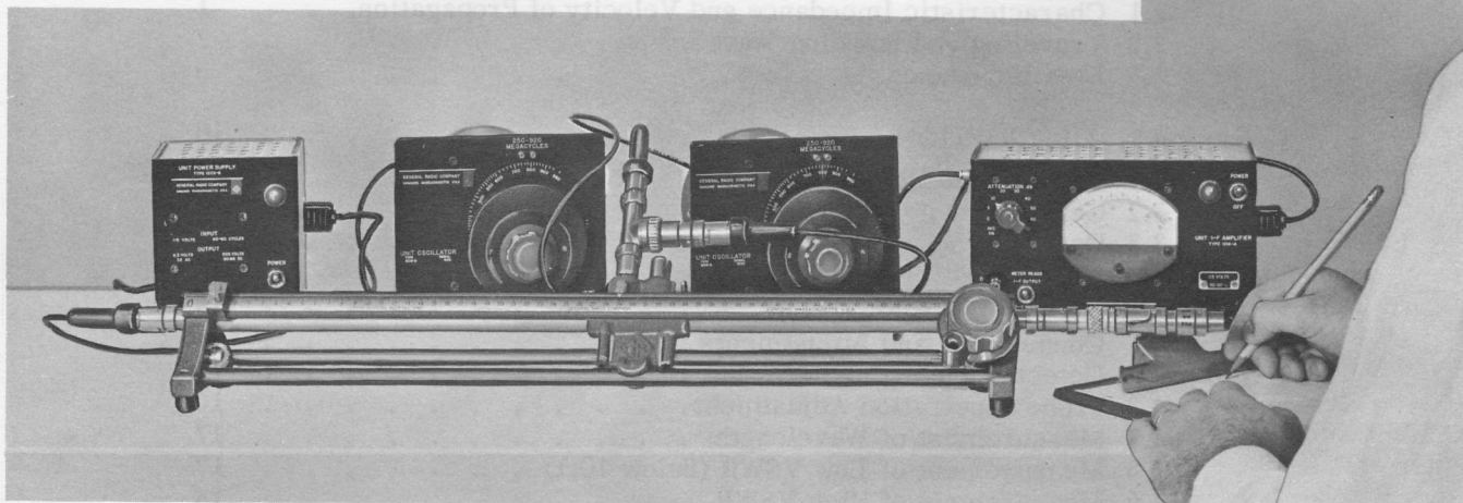
Figure 1. The Type 874-LBA Slotted Line and the Type 874-W50, 50-ohm Termination Unit are shown connected for the measurement of the VSWR of Type 874-QN Adaptors. These adaptors are used to connect components fitted with type N Connectors to devices fitted with Type 874 Connectors.
