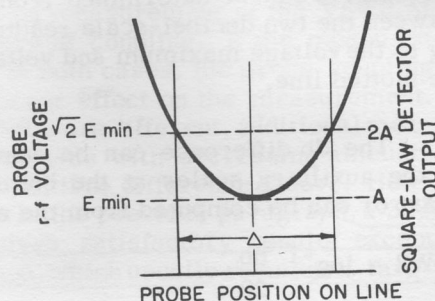
Figure 15. Method of measuring the width of the voltage minimum for VSWR determinations when the VSWR is high.
