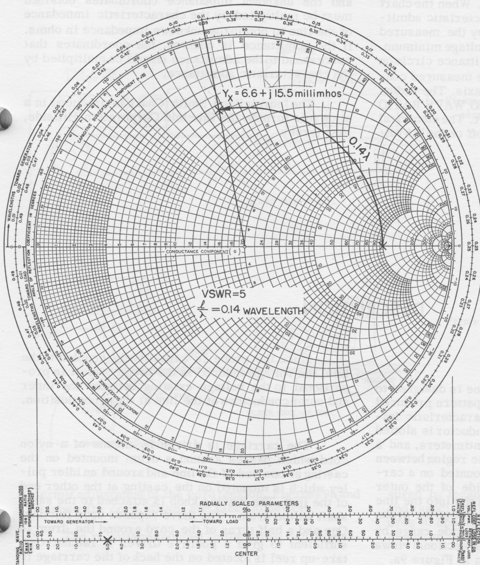
Figure 8. Example of the calculation of the unknown admittance from measurements of the VSWR and the position of a voltage minimum, using the Smith Chart drawn for admittance measurements on lines having characteristic admittances of 20 millimhos (50 ohms).
