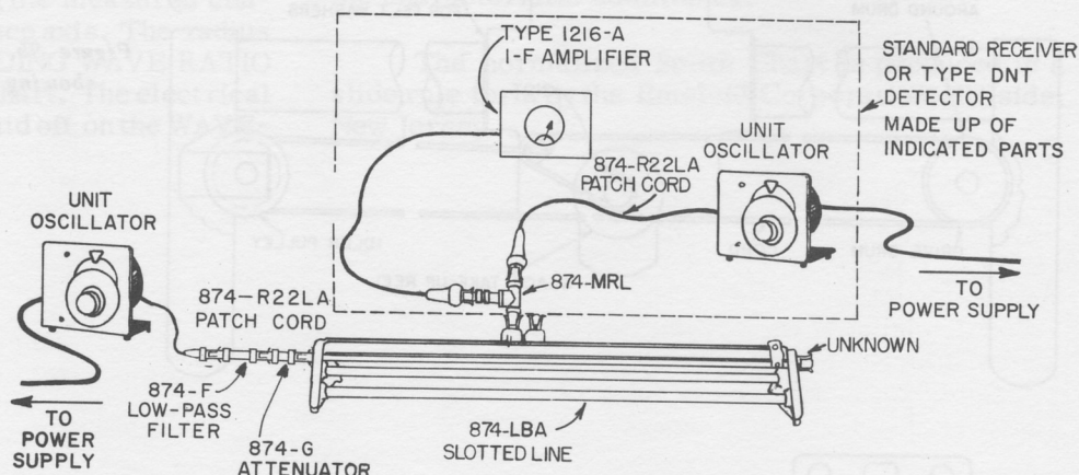
Figure 12. Use of an unmodulated source and a superheterodyne detector or receiver for measurements with the Type 874-LBA Slotted Line.
